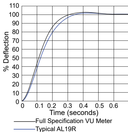
Comparison of Vintage AL / VU response
